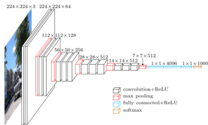
deep learning
